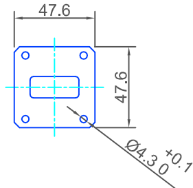
UG-51 /U (MIL-F-3922/53-002)
