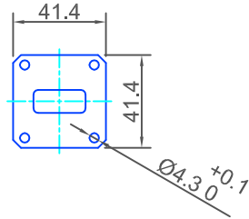
UG-39 /U (MIL-F-3922/53-001)
