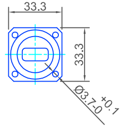
UG-419/U Modified MIL-F-3922/53-005 Modified
