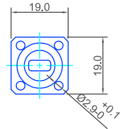
22Y SEALING GROOVE
