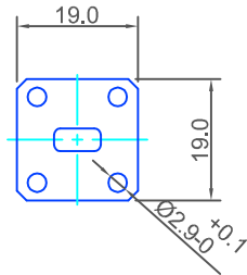
22B COVER / PLAIN
